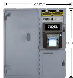
Tidel Series 4 with Standard Side Vault
